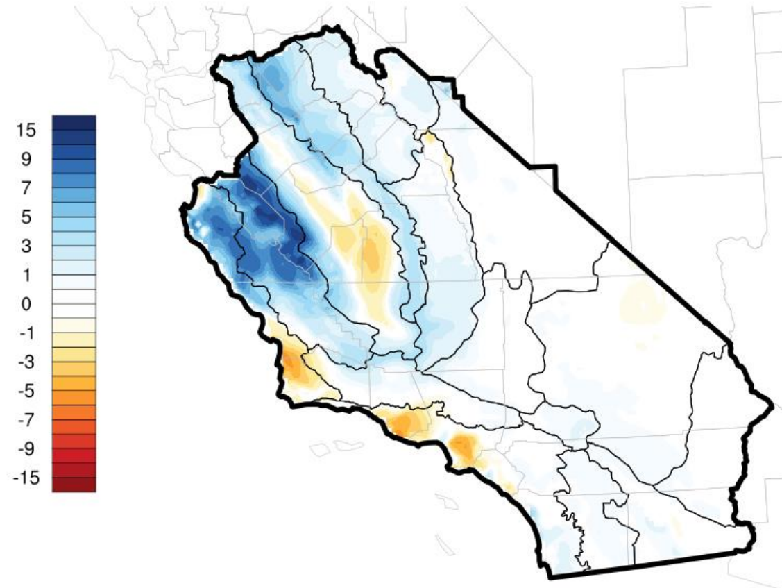
FM10 Hour change (%) from Yesterday
