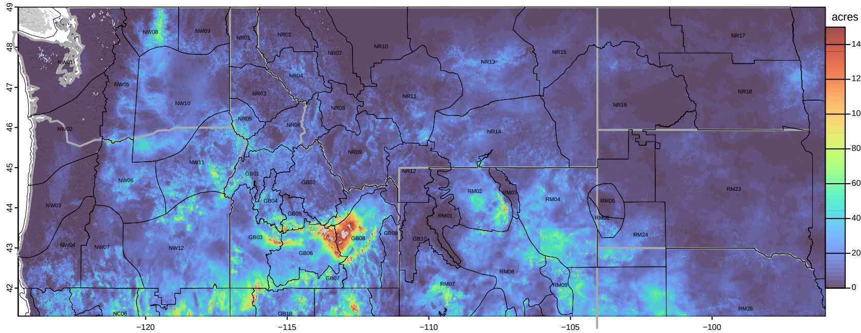
20260813 potential acres fire growth
