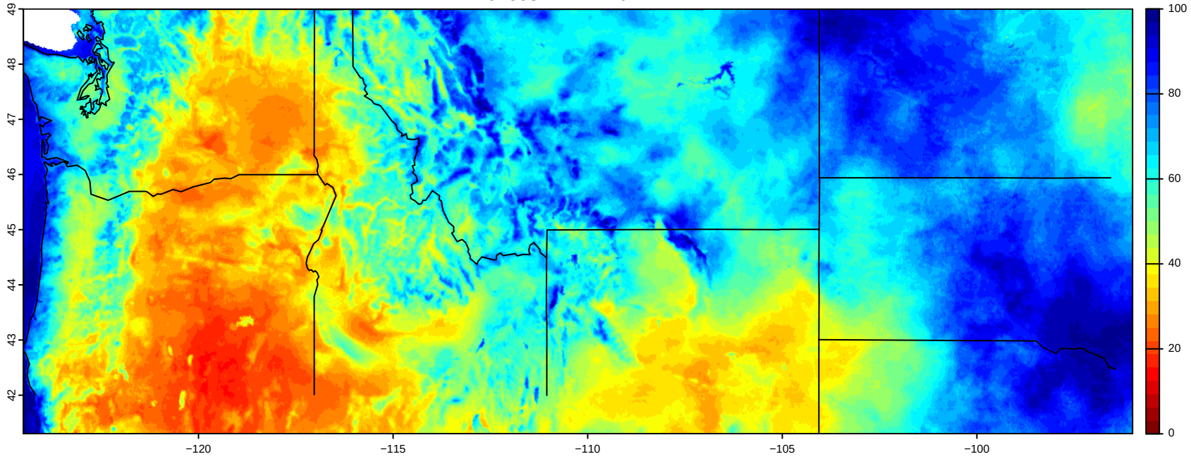
20260814 Minimum RH
