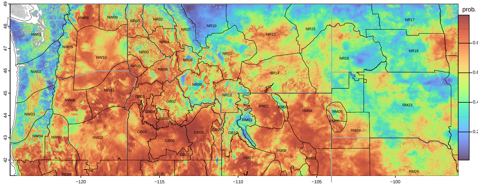
20260813 Probability. of fire spread > 70 acres
