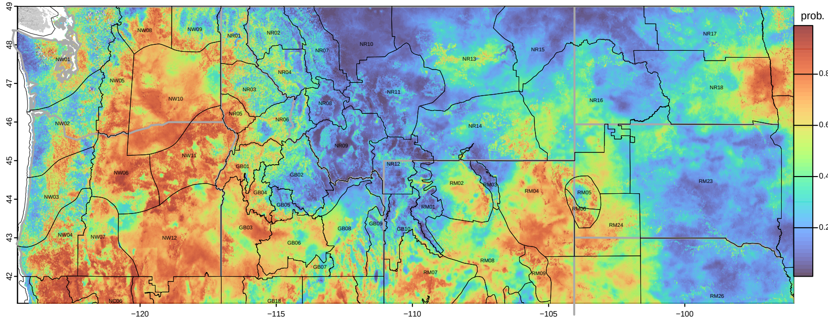
20260814 Probability. of fire spread > 70 acres
