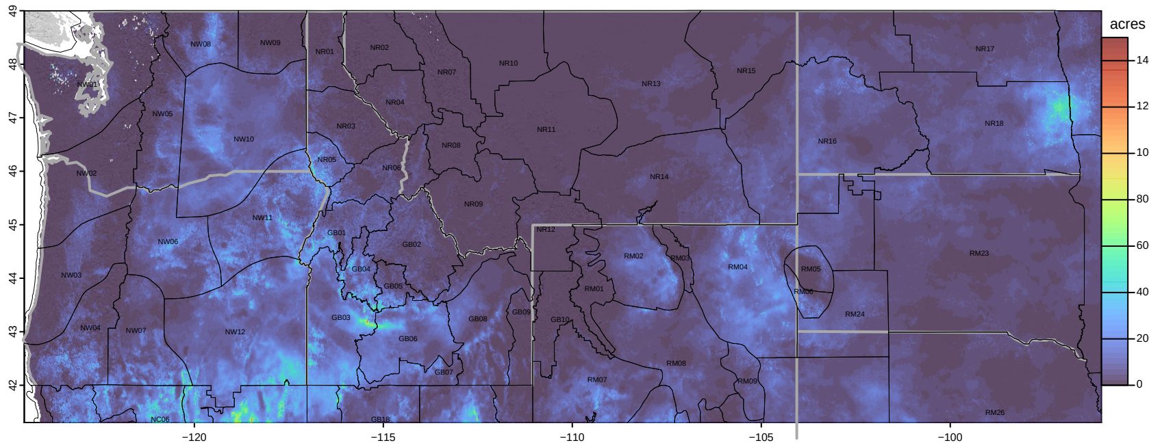
20260814 potential acres fire growth
