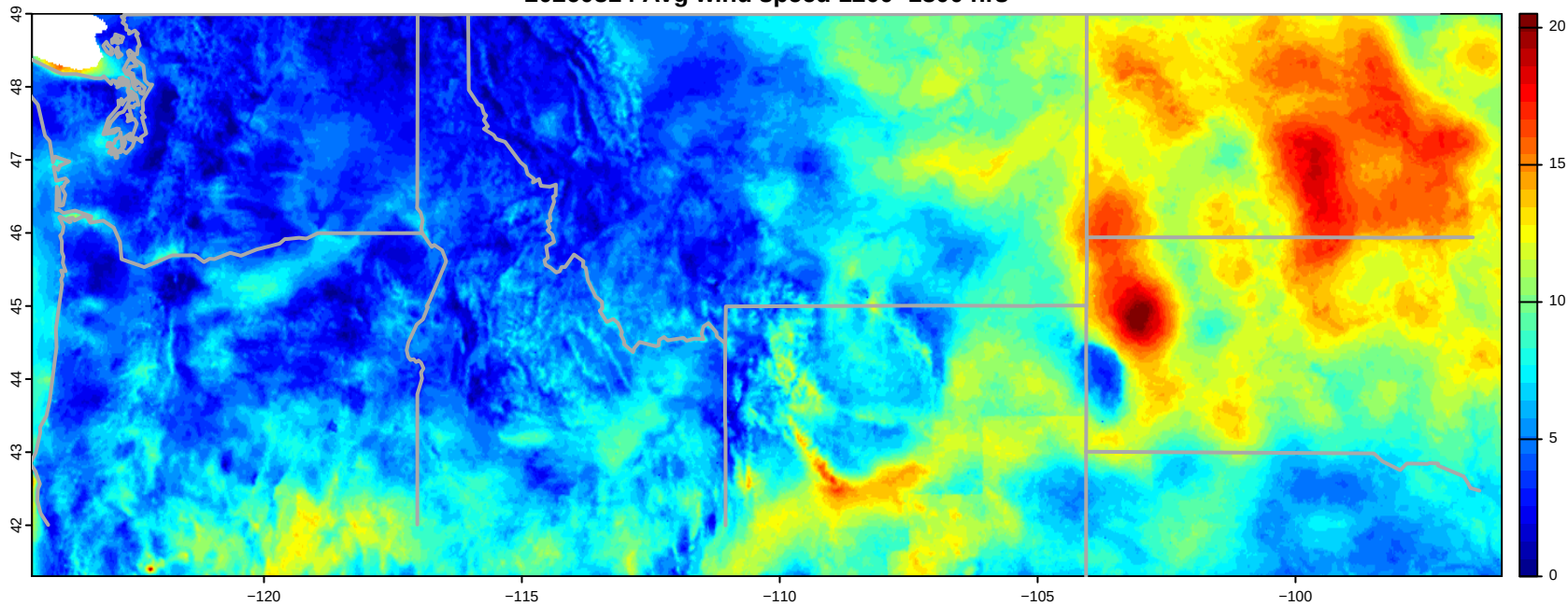
20260814 Avg wind speed 1200–1800 hrs
