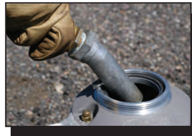
Figure 101—When a drip torch is filled properly, the pump nozzle touches the container, preventing sparks from static electricity generated by flowing fuel.
