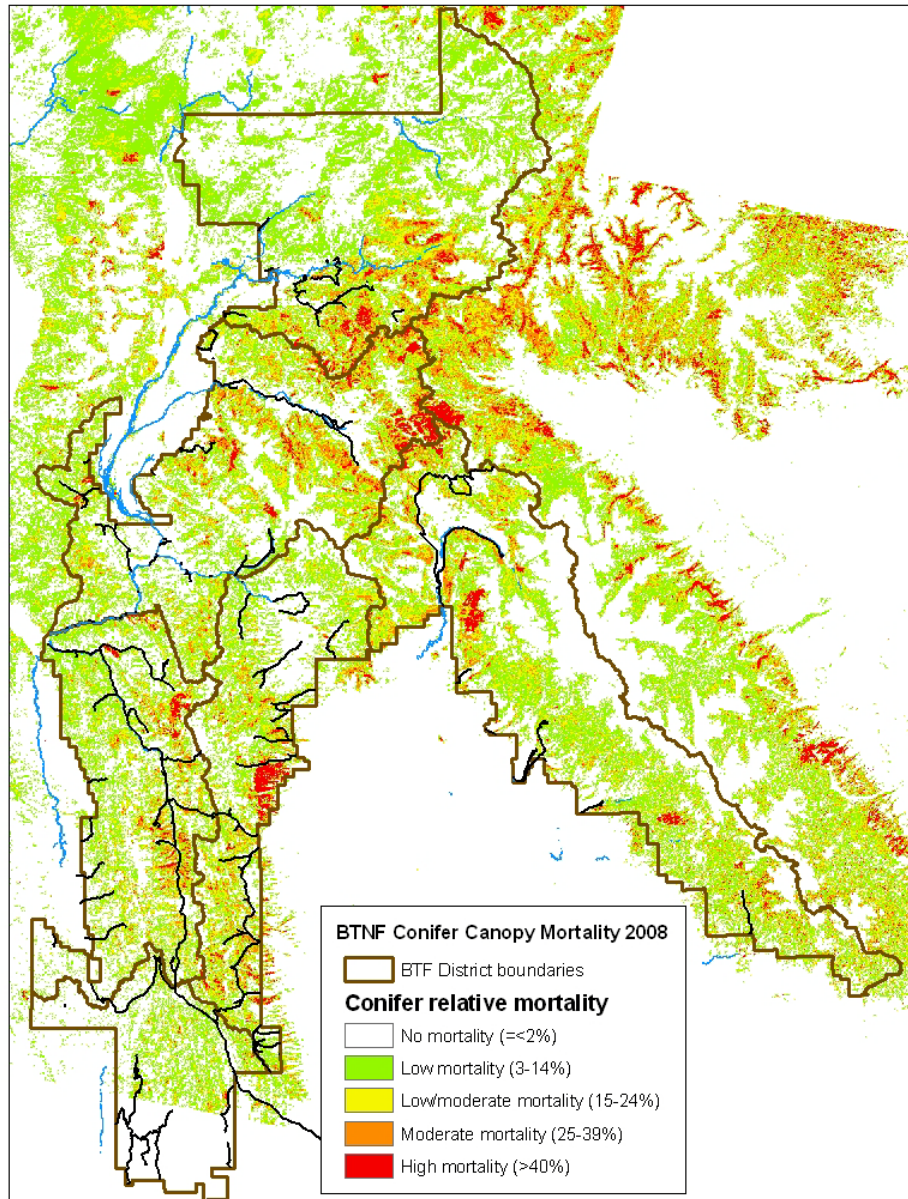
Figure 3.1.2.2 Bridger-Teton conifer mortality (2008)
