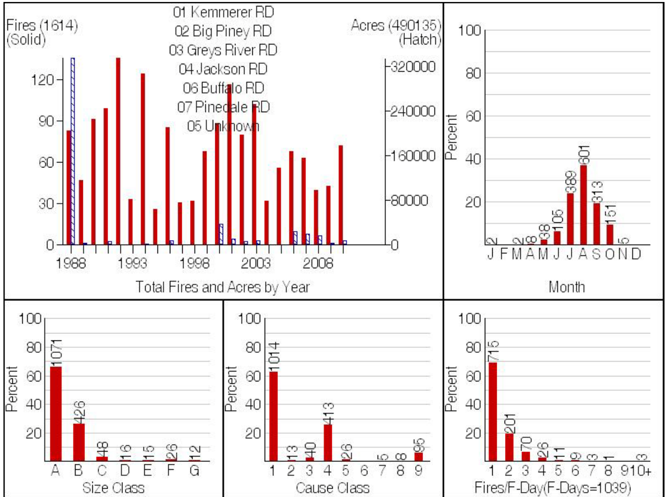
Figure 3.1.2.1: Historical fire occurrence on the Bridger-Teton NF, 1988-2010
